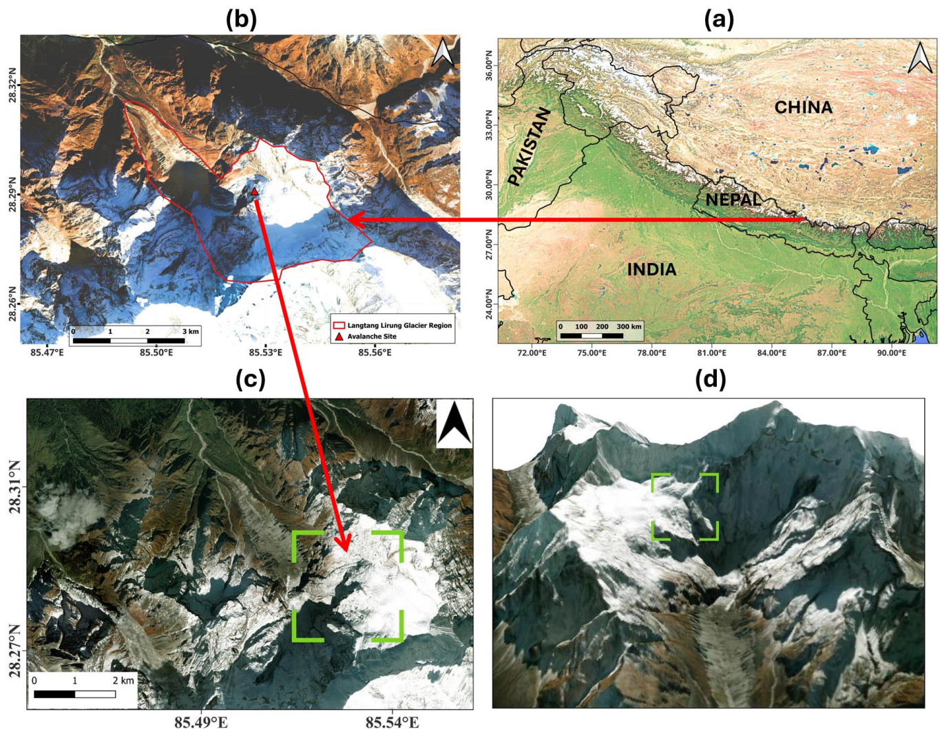
Figure 1. Geographic location and topographic setting of the Langtang Lirung study area: (a) study area location within Nepal and its regional context; (b) Langtang Lirung Glacier and the identified avalanche source area; (c) regional geomorphic setting highlighting the reported avalanche initiation zone (green zone); and (d) three-dimensional view of the northern slope of Langtang Lirung. Source: Authors.
