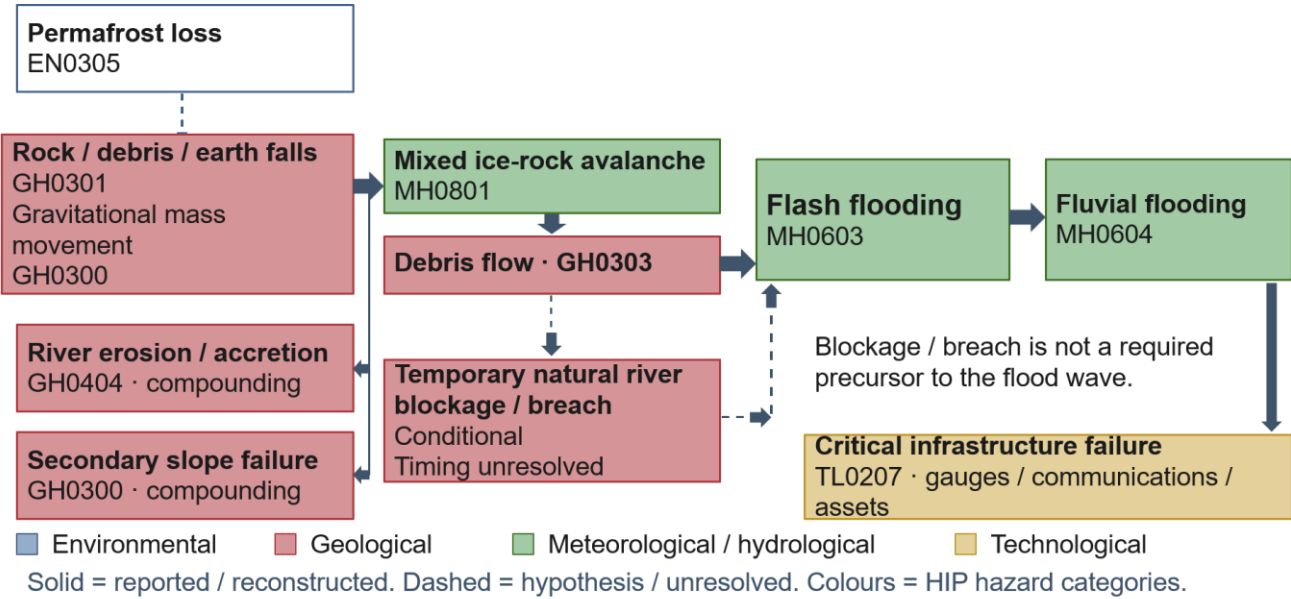
Figure 3. Hazard Information Profile classification of the Langtang Lirung cascade (Source: Authors).
