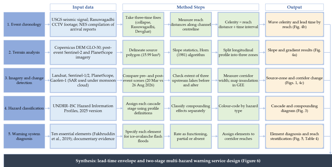
Figure 2. Analytical framework for reconstruction of the Langtang Lirung cascade and assessment of its implications for multi-hazard early warning [12,14,15].
